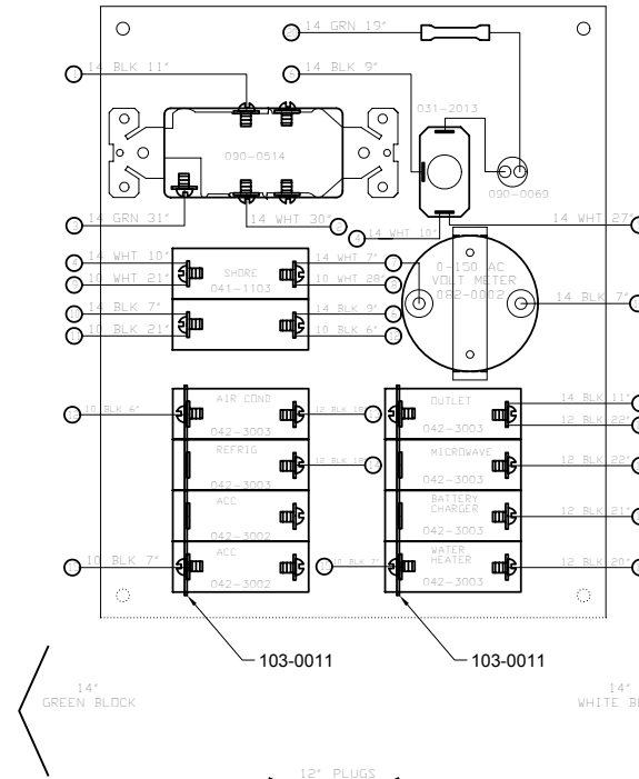
PLUG "A" 3 POS 25A LG CAP HSG 052-2011 W/LARGE PINS (3) 052-2019 PIN 10-12GA
