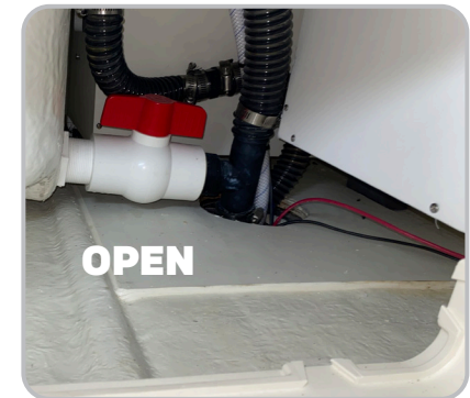
Transom Walkthrough Step Seacock Access Hatch
