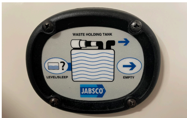
Jabsco Tank Monitor installed with Overboard Discharge Feature
