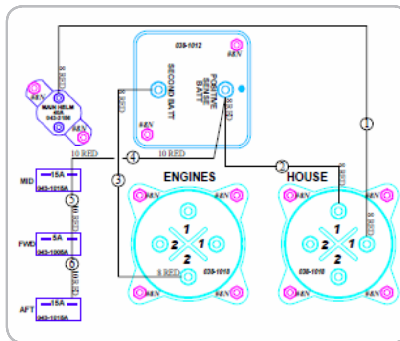
Back View With Wiring
